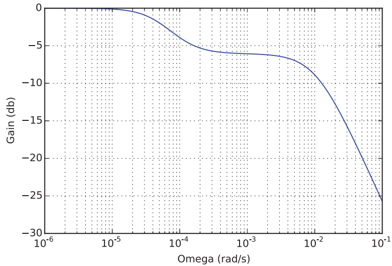
FIGURE 10 – Diagramme de Bode sans isolation
